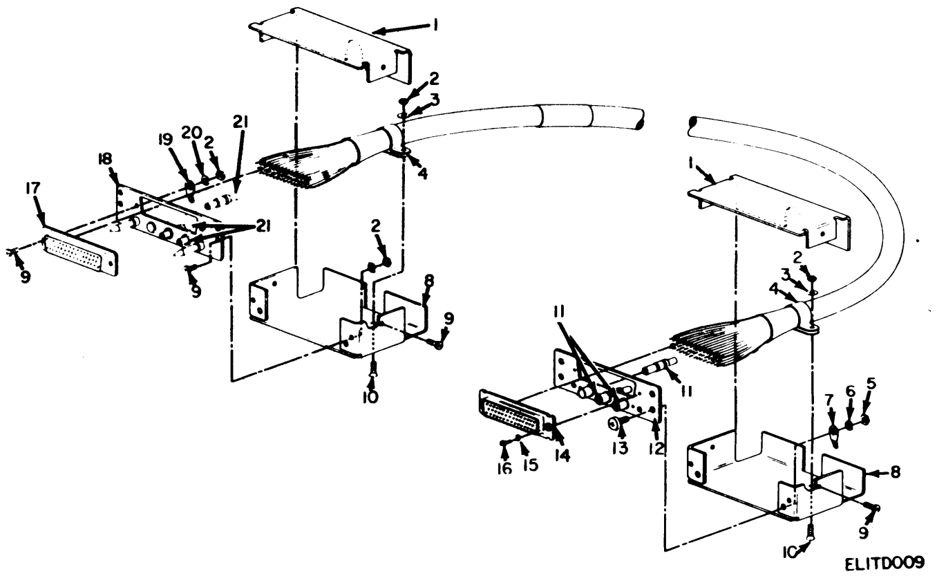
Figure 9. Cable Assembly CX-9072/ARC-54.
