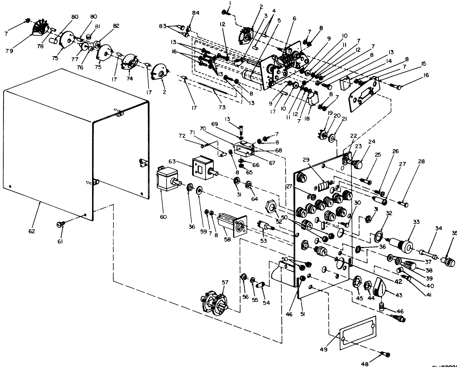
Figure 19. Front Panel Assembly SMB 50493.
