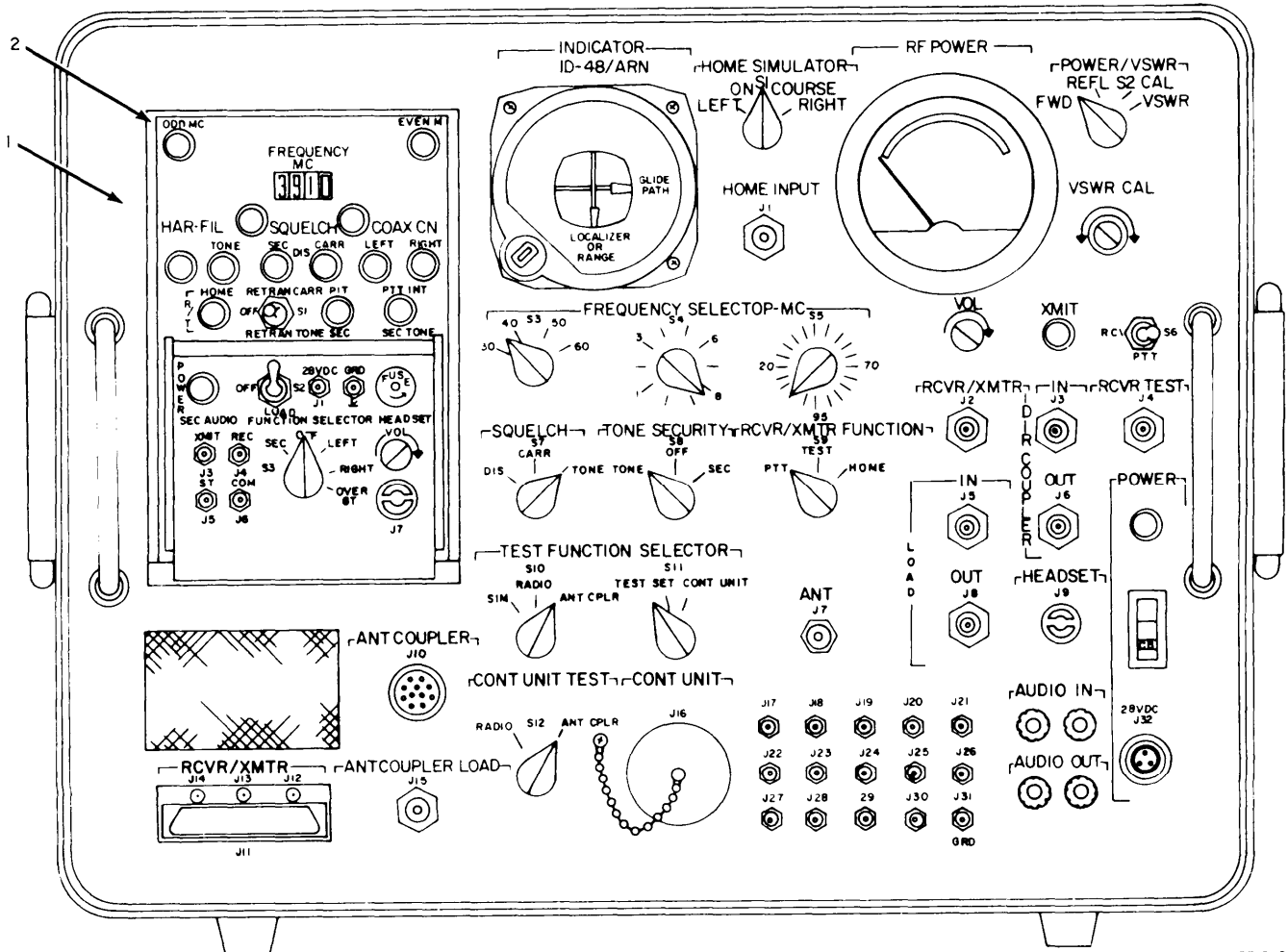
Figure 12. Test Set, Radio TS-1967/ARC-54.
