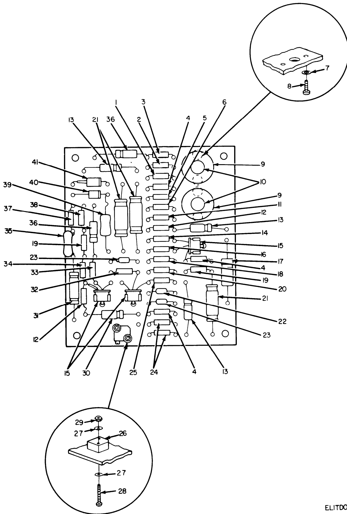
Figure 15. Audio Amplifier A1.
