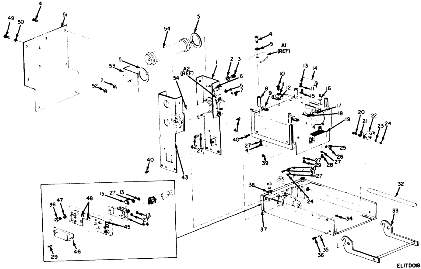
Figure 17. Simulator, Test Set SM-349/ARC-54, Chassis Assembly.
