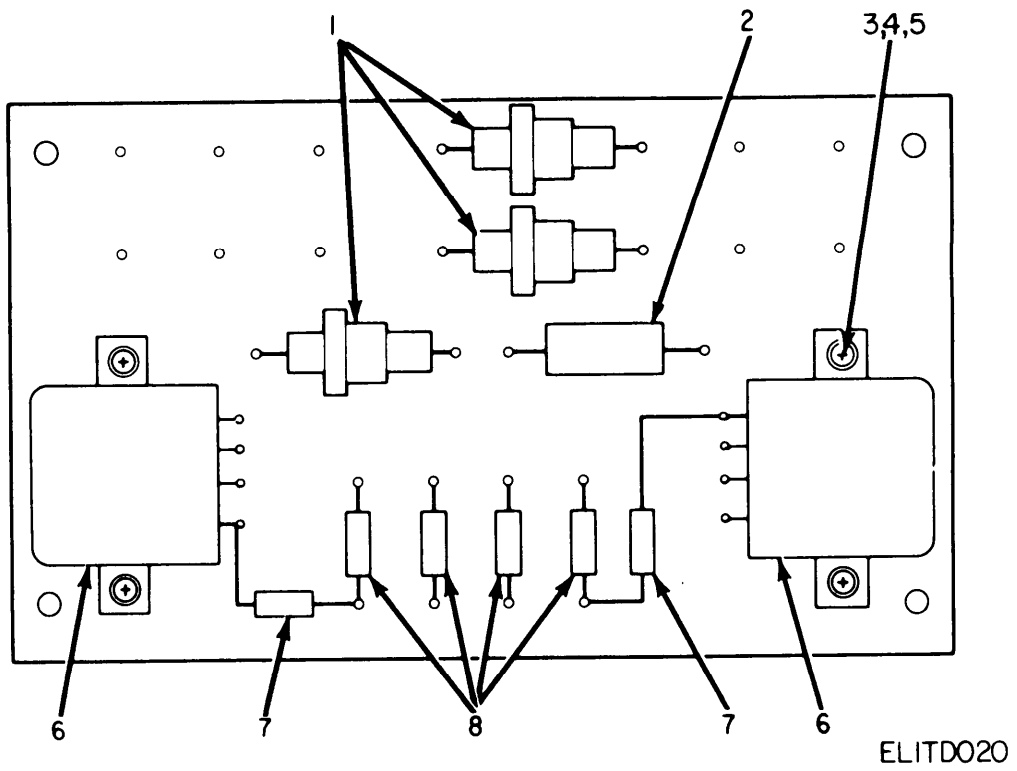
Figure 18. Electronic Component Assembly A2.
