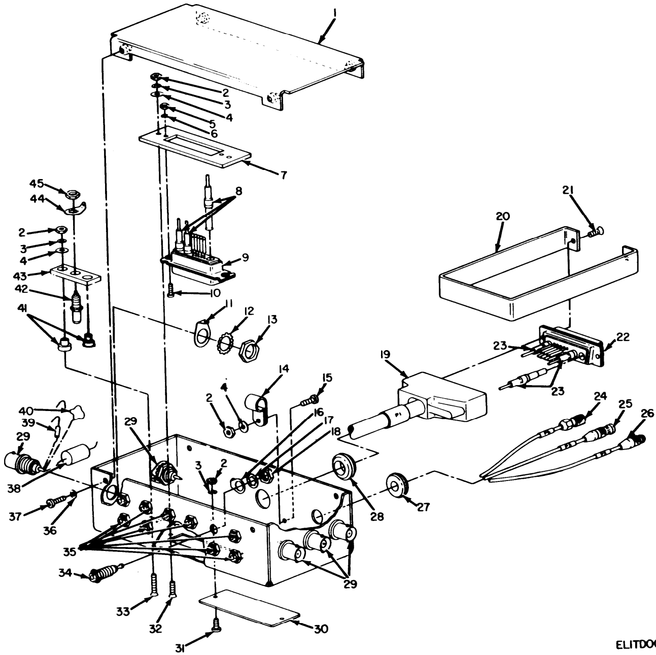
Figure 3. Extender Module MX-4931/ARC-54.
