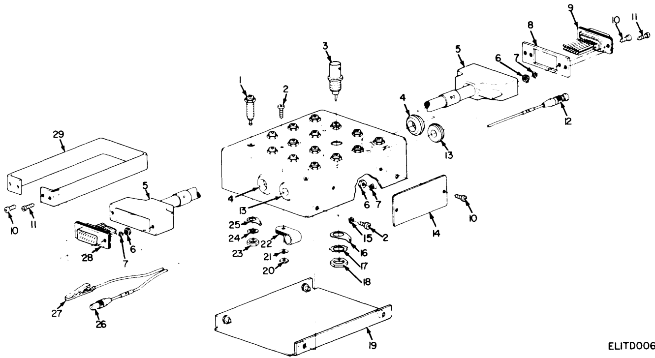
Figure 6. Extender Module MX-4934/ARC-54.
