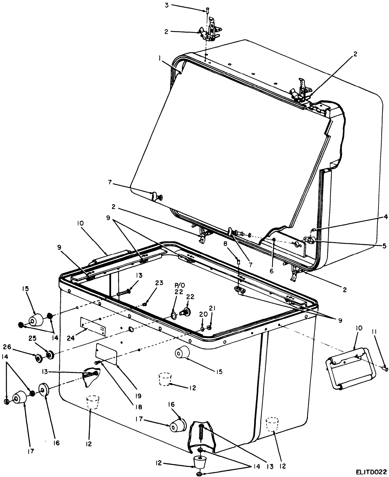
Figure 20. Case, Maintenance Kit CW-711/ARC-54.
