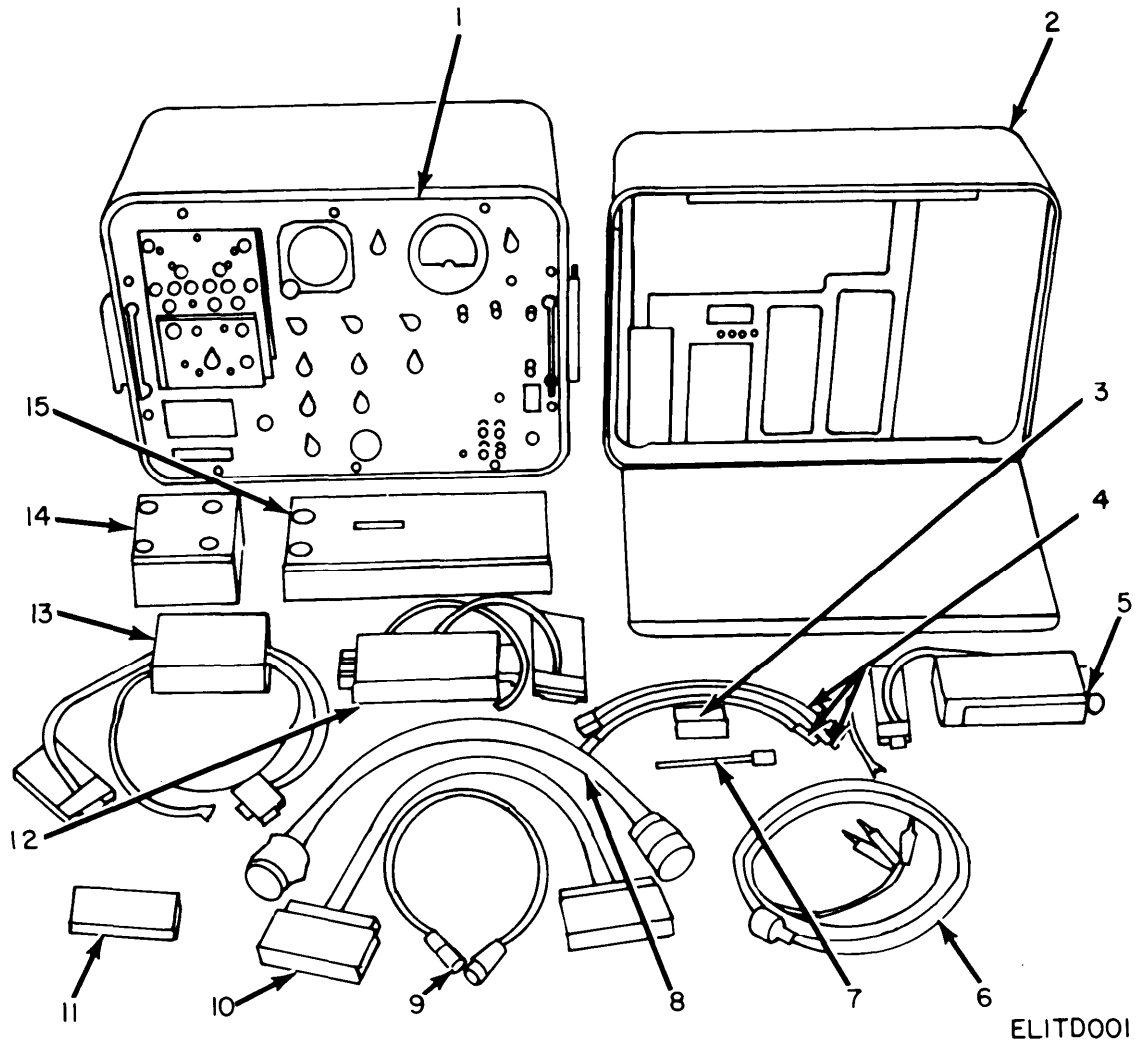
Figure 1. Maintenance Kit, Electronic Equipment MK-733/ARC-54.
