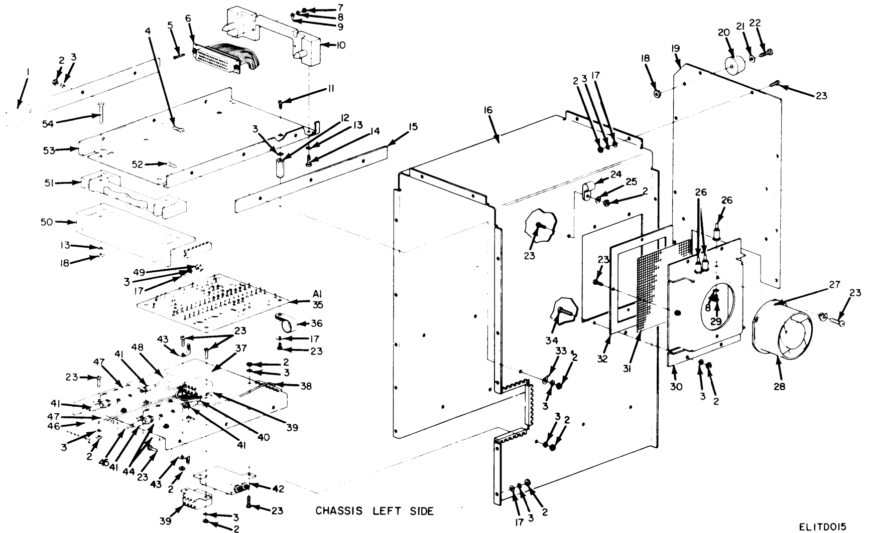
Figure 14. Front Panel Assembly (SMB-504958), Chassis (Sheet 1 of 2).
