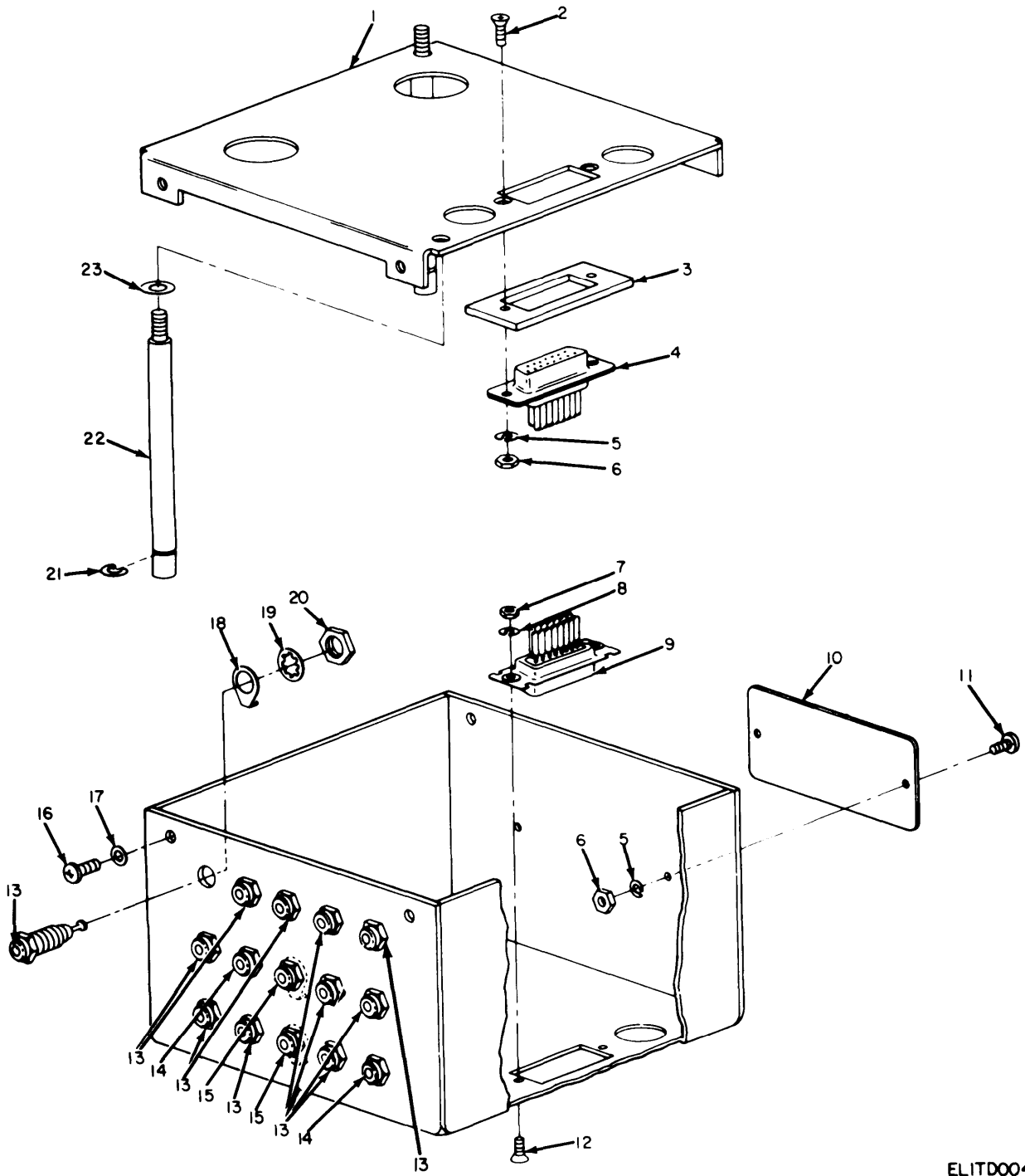
Figure 4. Extender Module MX-4932//ARC-54.
