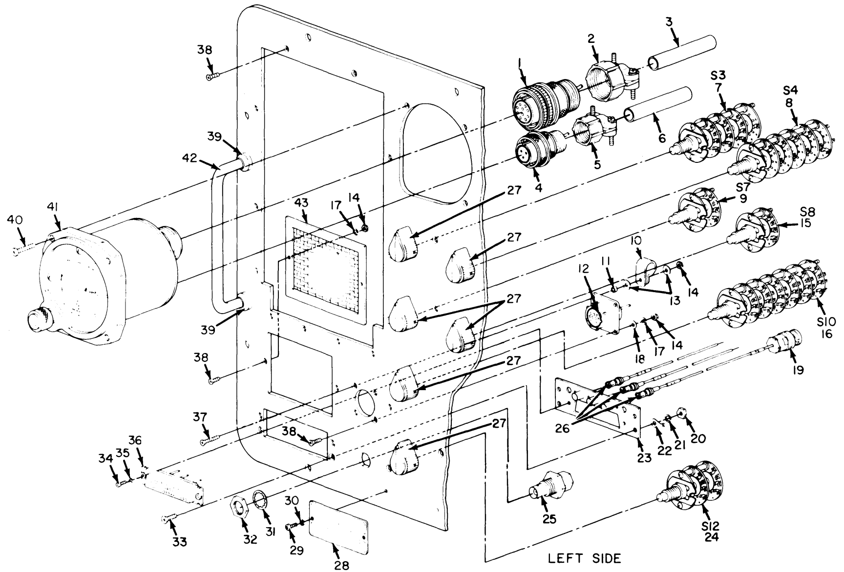
Figure 13. Front Panel Assembly (SMB-504958) (Sheet 1 of 2).
