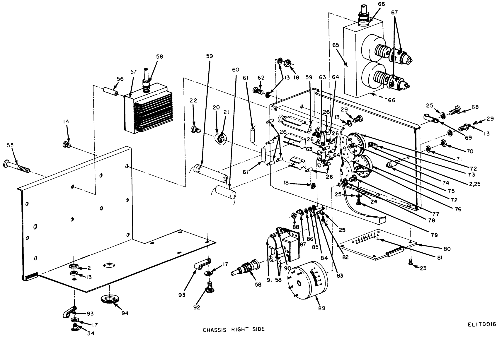
Figure 14. Front Panel Assembly (SMB-504958), Chassis (Sheet 2 of 2).
