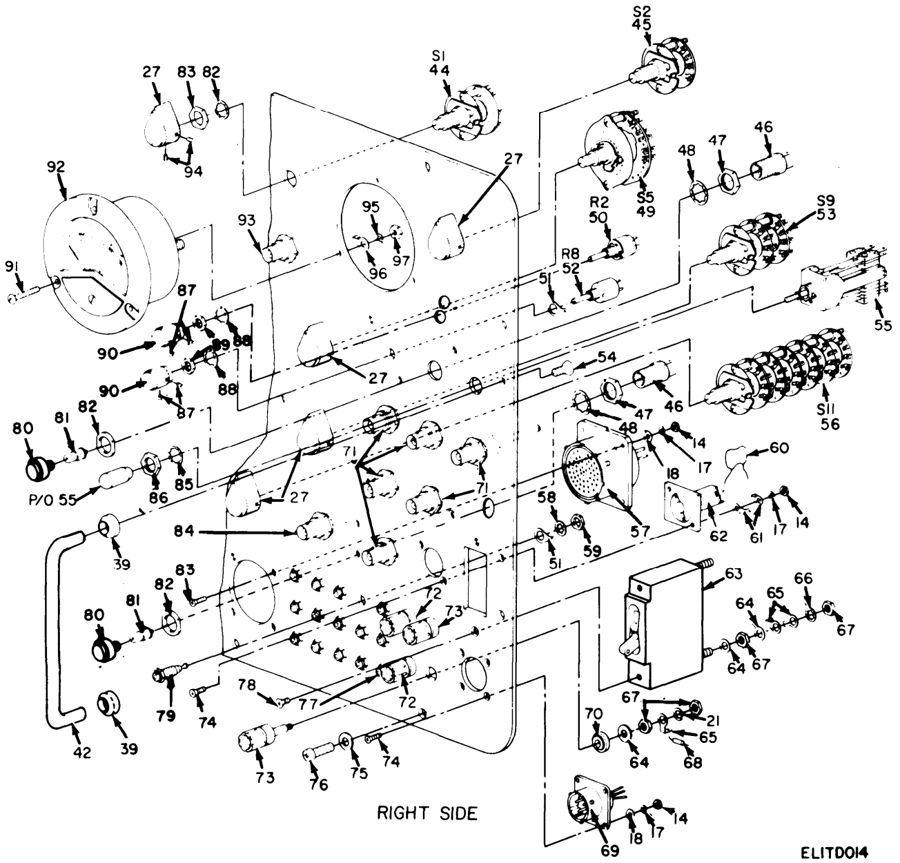
Figure 13. Front Panel Assembly (SMB-504958) (Sheet 2 of 2).
