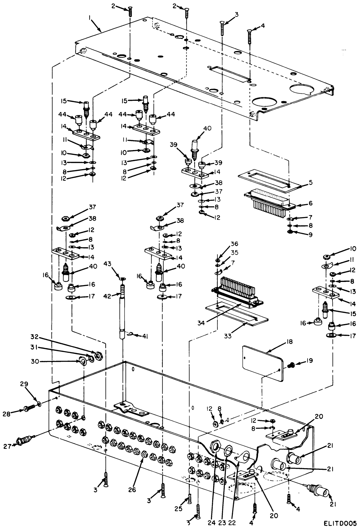
Figure 5. Extender Module MX-4933/ARC-54.
