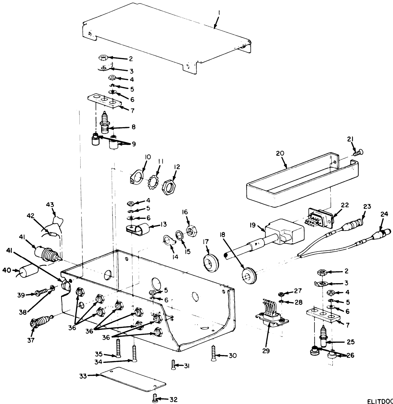
Figure 2. Extender Module MX-4930/ARC-54.
