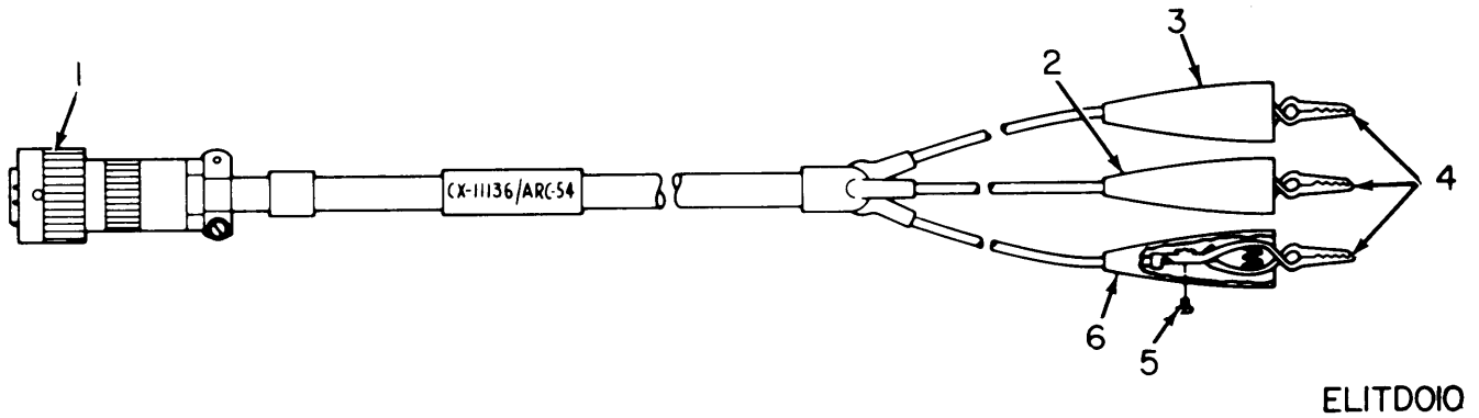
Figure 10. Cable Assembly CX-11136/ARC-54.
